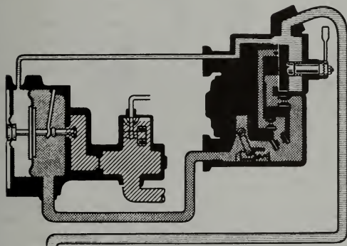
FIGURE 3-28. Manual mixture control in idle cutoff.
